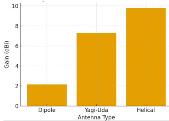
Figure 6: Gains Comparison of Antennas in FM Transmission
