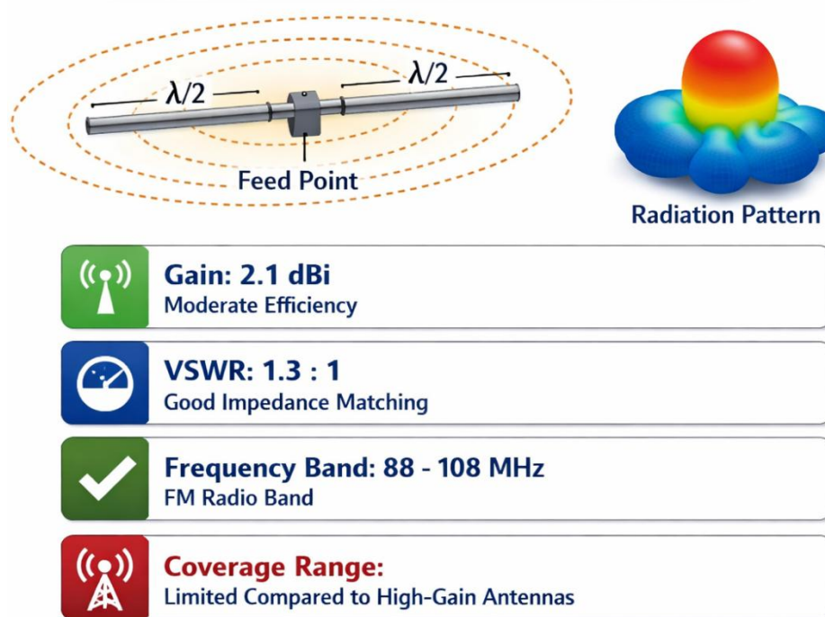
Figure 7: Half-Wave Dipole Antenna Results
