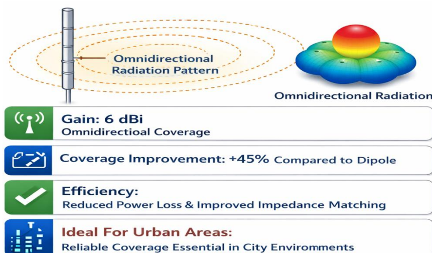
Figure 9: Collinear Array Antenna Results
