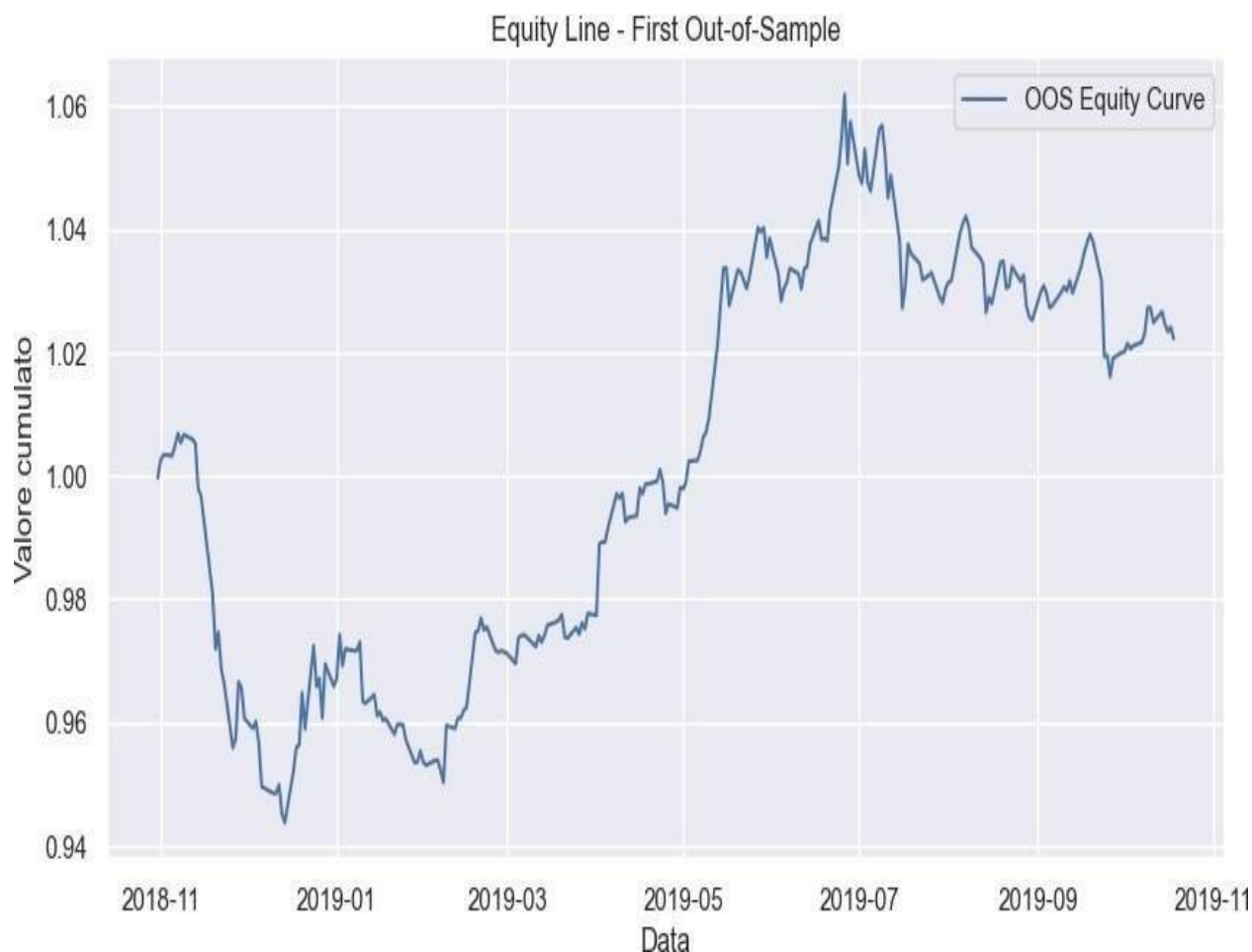
Figure 2: Equity curve for the first one-year out-of-sample period.
