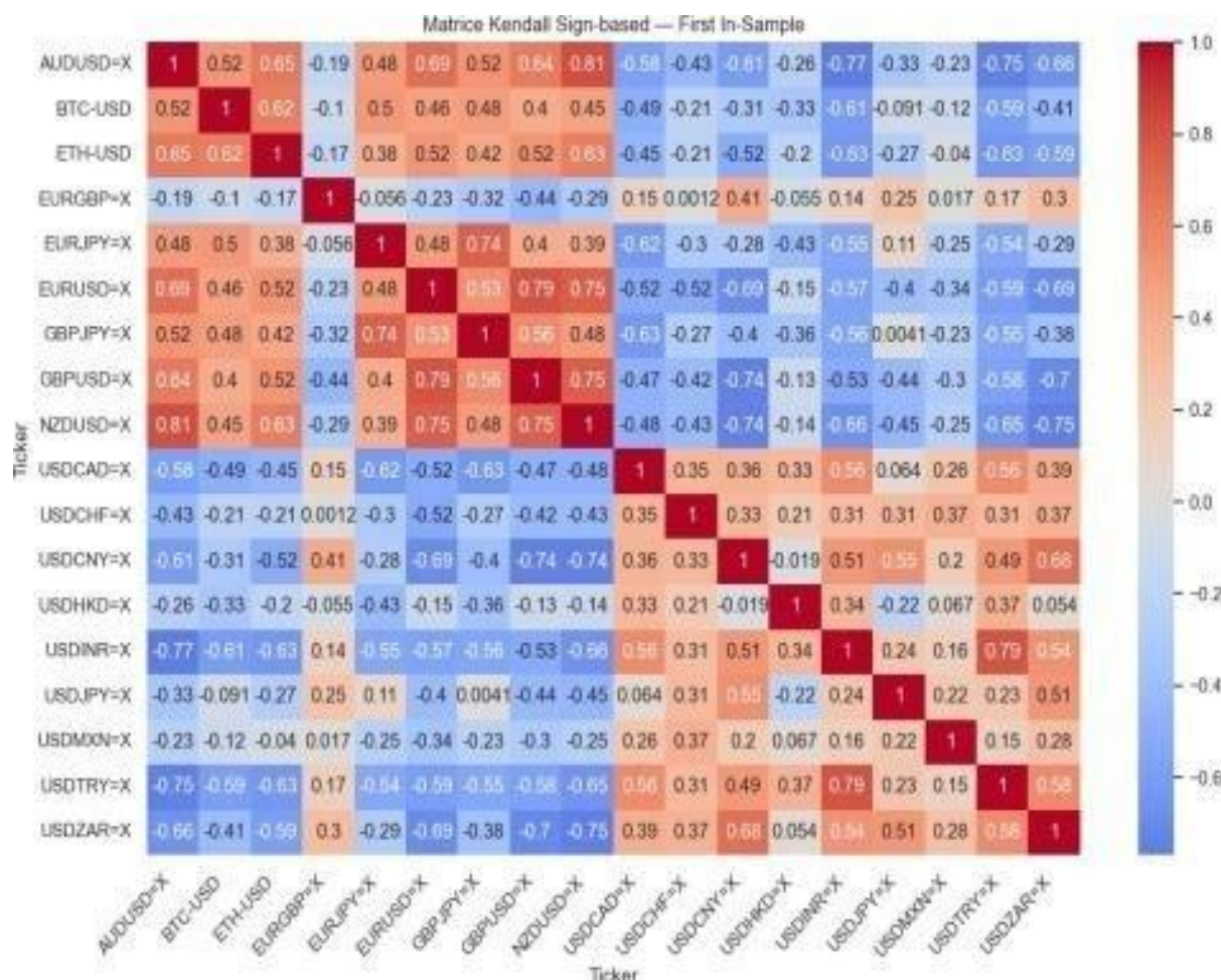
Figure 1: Sign-based Kendall correlation matrix for the first in-sample window.
