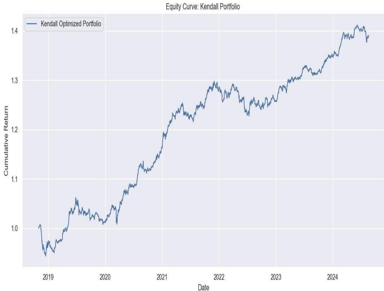
Figure 3: Kendall-optimized portfolio over the full evaluation period.
