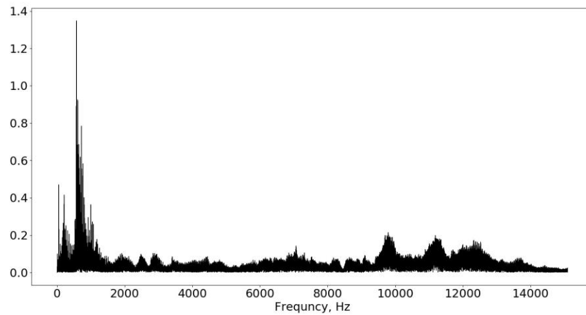
Figure 6. Spectrum of the signal. The normal spring is mounted on the exhaust valve.
