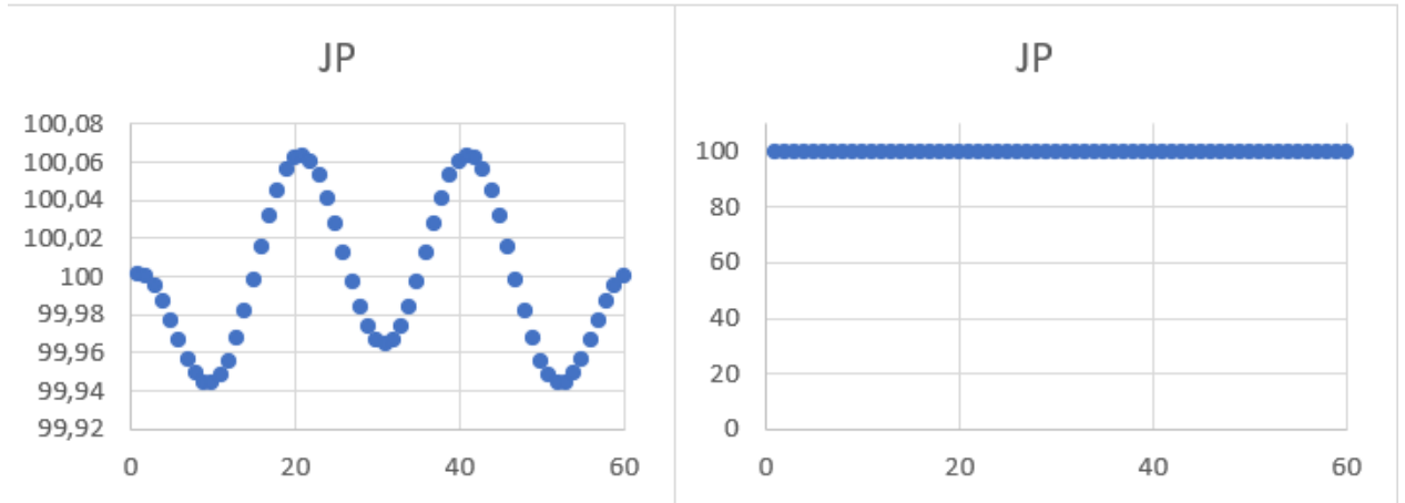
Figure 11: Values of J_p returned by program for 15 flux measurements
