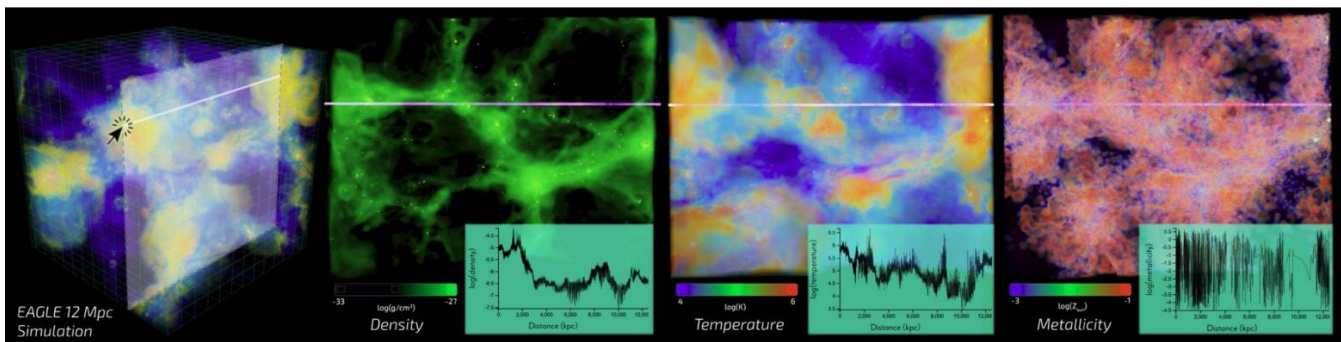
Fig. 1 Hydrodynamical simulation [4]
