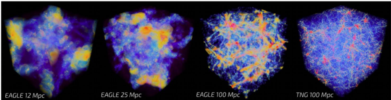
Fig. 2: EAGLE simulation [4]
