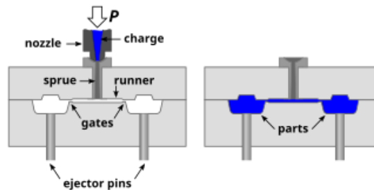
Fig 1: Simplified Diagram Of The Process (Photo Source – Wikipedia )
