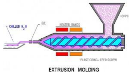
Fig 3: Extrusion Molding (Photo Source – Engineers gallery )
