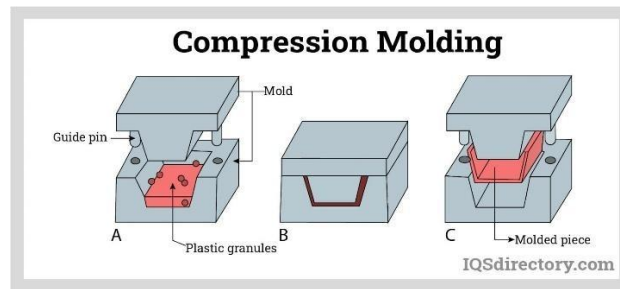
Fig 6: Compression Molding (Photo Source – Iqsdirectory )
