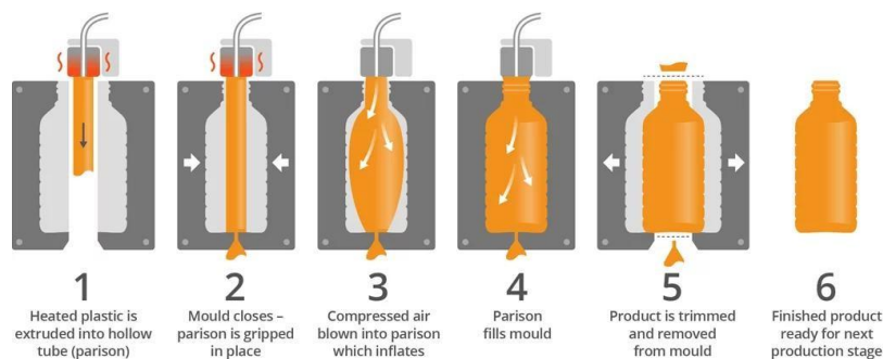
Fig 5: Blow Molding (Photo Source – Robinson packaging )
